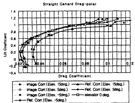
Fig. 12 Drag-polar for straight canard
