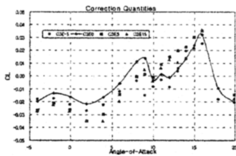
Fig. 8 Lift coefficient correction quantities
