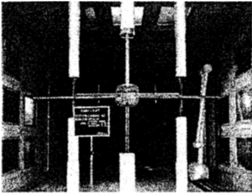
Fig. 2 Normal installation with image system
