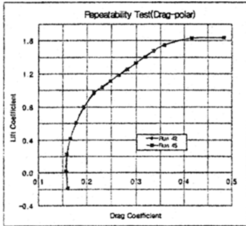
Fig. 5 Drag-polar repeatability
