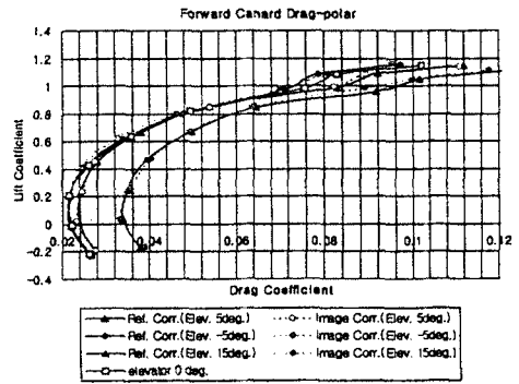
Fig. 11 Drag-polar for forward-swept canard
