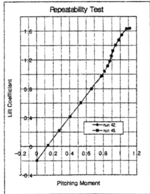
Fig. 6 Lift and P. M. repeatability
